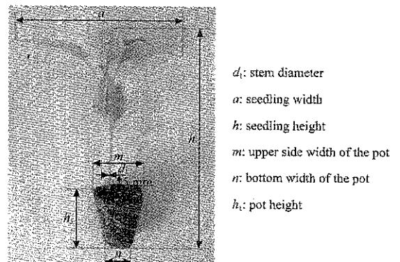
Figure 5 Morphological parameters of the pot seedlings
