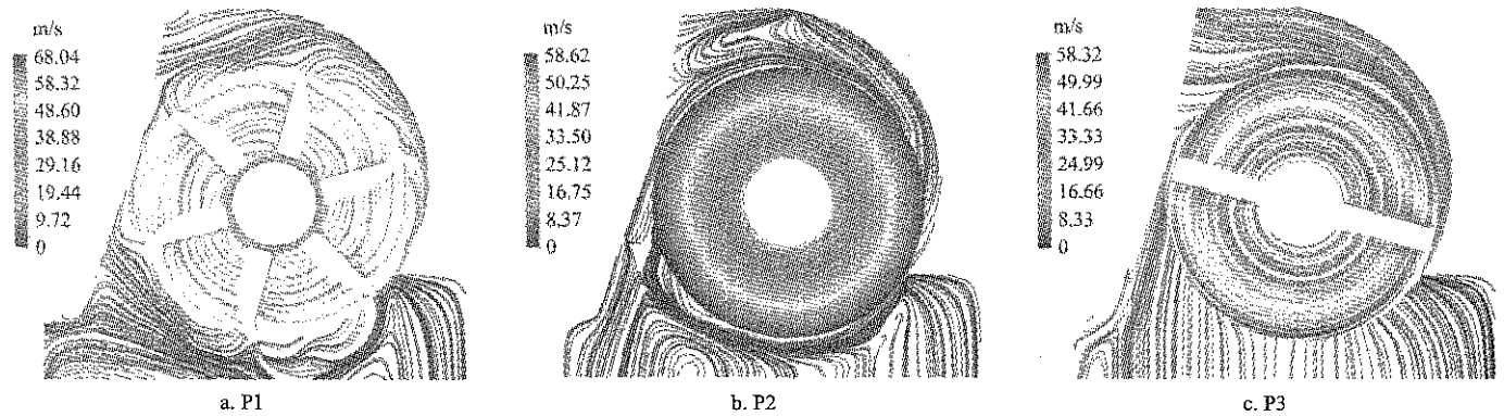
Figure 18 Streamlines on sampling plans in the chopping chamber with guide vanes
