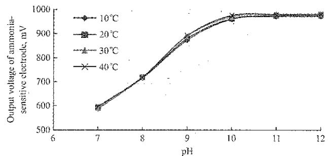
Figure 7 Variations in the output voltage of the ammonia-sensitive electrode transmitter with respect to pH values at different temperatures
