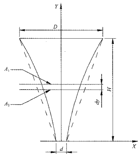
Figure 1 Hyperbolic funnel
