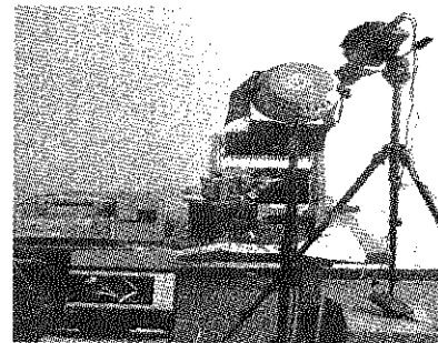
Figure 8 Test bed
