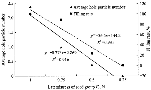
Figure 5 Influence of lateral width of seed-filling room on seeding performance
