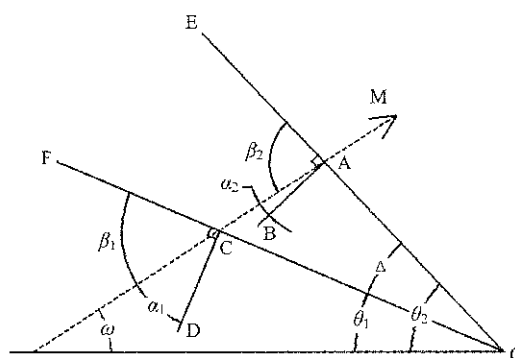
Figure 4 Analysis of collision theory between soil and arc-shaped shell
