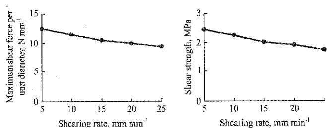
Figure 7 Relationship between shear properties and shearing rate
