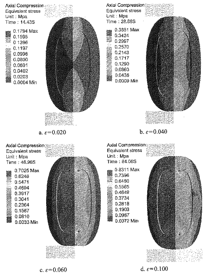
Figure 10 Stress nephogram of axial compression
