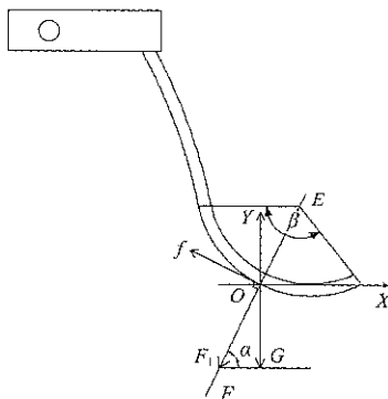
Figure 6 Force analysis of the rice straw at the end of blocking rice straw device
