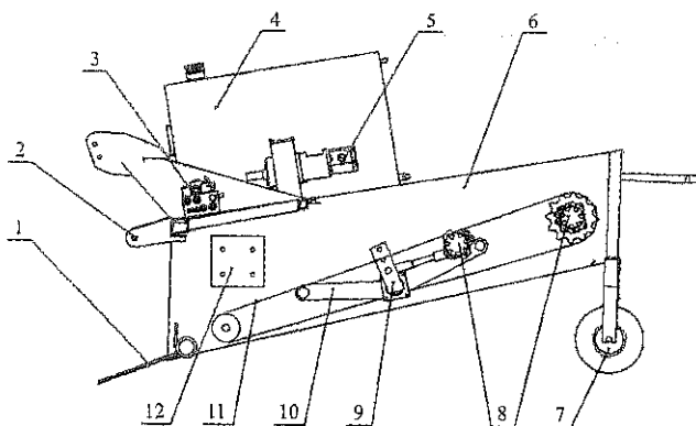
1. Digging device 2. Traction frame 3. Hydraulic proportion valve 4. Hydraulic fluid chamber 5. Hydraulic pump 6. Body frame 7. Land wheel 8. Hydraulic motor 9. Adjustments panel 10. V-shaped vibration device 11. Closed rotary sieve 12. Electronic control system
