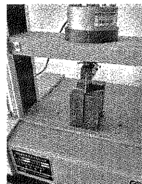
Figure 4 Shear test of sweet potato vine
