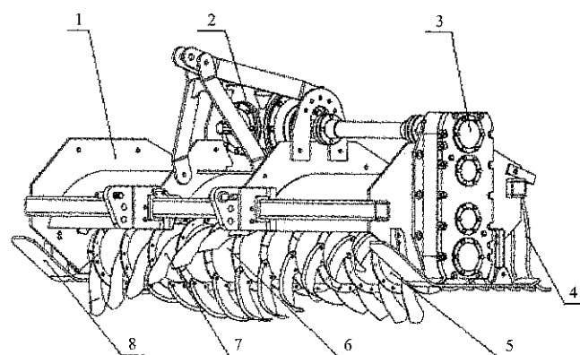
1. Frame 2. Central reducer 3. Side reduce 4. Blocking rice straw device 5. Knife roller 6. Knife seat 7. Knife 8. Limiting the depth plank
