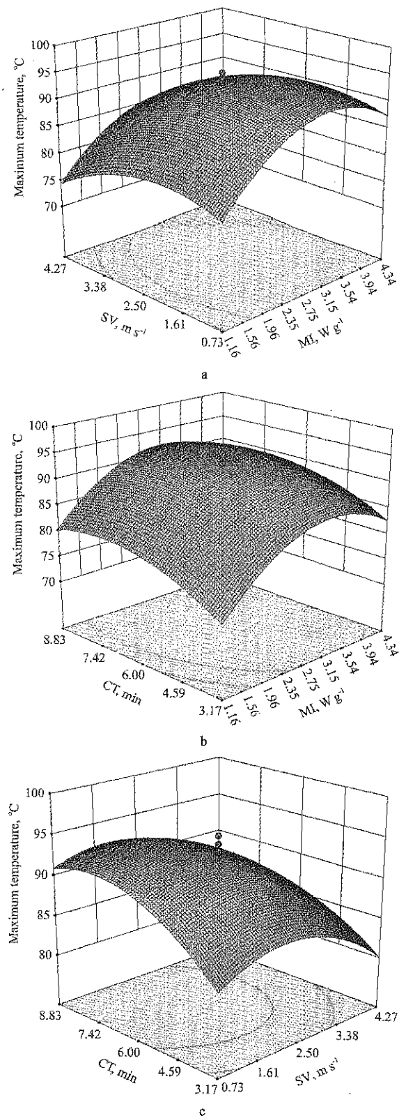
Figure 4 Effects of microwave drying conditions on the maximum temperature of GBR
