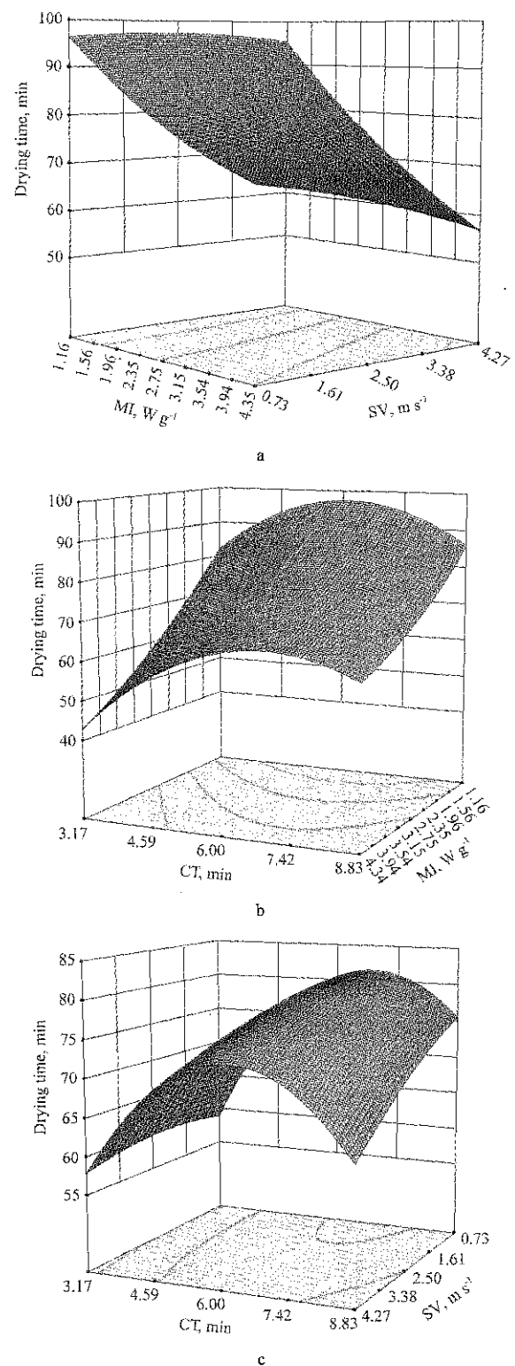
Figure 2 Effect of microwave drying conditions on the drying time of GBR
