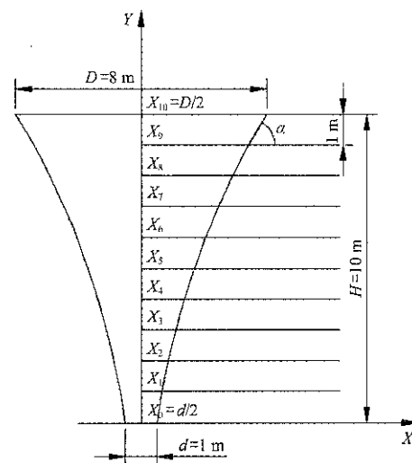
Figure 2 Subsection sketch map of the hyperbolic funnel
