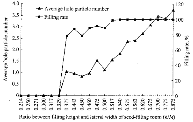
Figure 7 Influence of ratio between filling height and lateral width of seed-filling room on seed-filling performance
