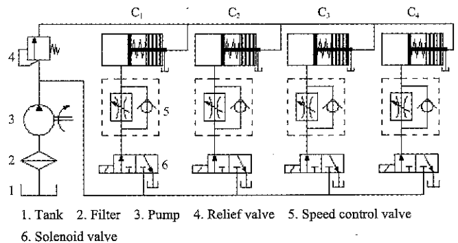
Figure 4 Principle diagram of hydraulic control for clutch
