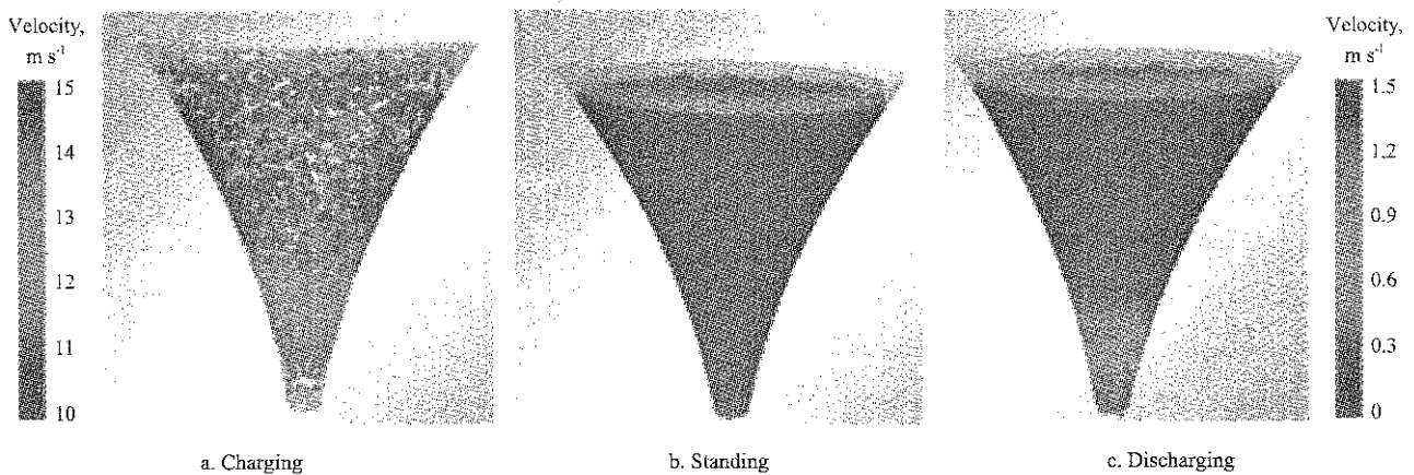
Figure 3 Charging and discharging processes of the hyperbolic funnel
