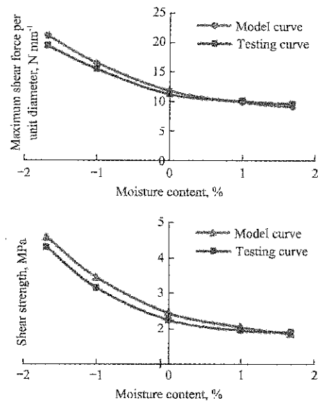
Figure 10 Shear property model verification of sweet potato vine
