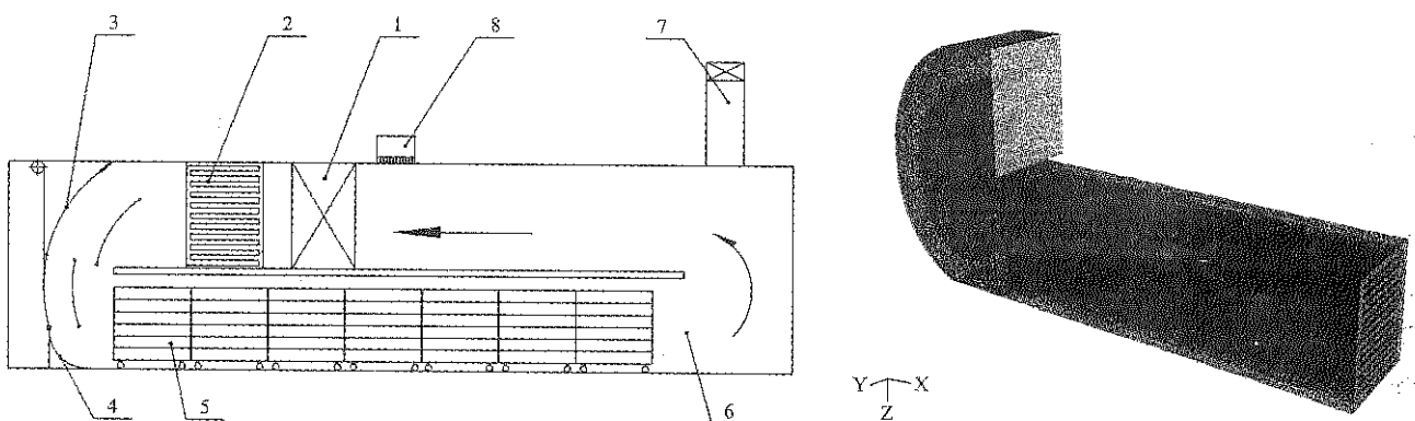
1. Axial flow fan 2. Steam heater 3. Removable guide plate 4. Fixed guide plate 5. Dryer wagon 6. Drying chamber 7. Moisture-removing exit 8. Fresh air inlet
