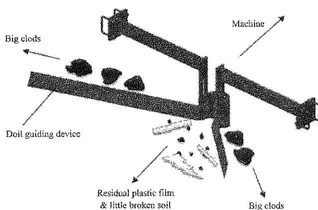
Figure 5 Operation principle diagram of soil-guiding device
