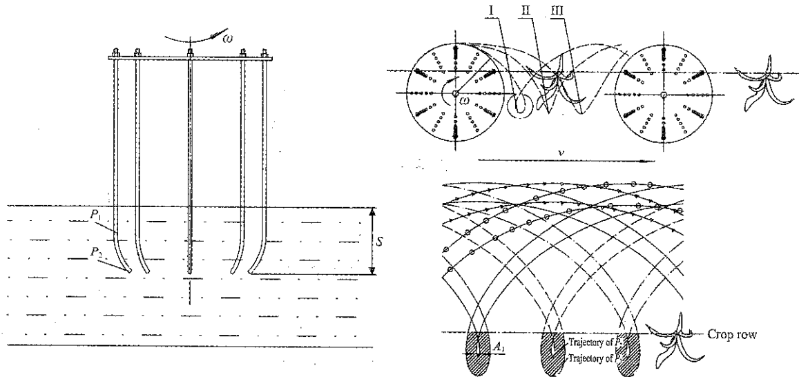
Note: P_1 and P_2 represent the two endpoints of arc-shaped segment of spring-tooth. I, II and III regions represent the weeding control areas of spring-tooth in different conditions, respectively. The circles and triangle represent the weeding control trajectories of spring-tooth in different conditions, respectively. A_1 is the minimum range of trajectories caused by two endpoints of spring-tooth. S is the distance from soil surface to spring-tooth end. v is the machine forward velocity. \omega is the cutter-disc rotational speed.
