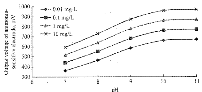
Figure 8 Variations of the ammonia-sensitive electrode transmitter output voltage with different pH concentrations
