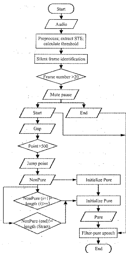
Figure 3 Fast filter algorithm
