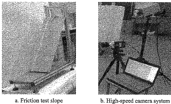
Figure 3 Seedling friction coefficient test device
