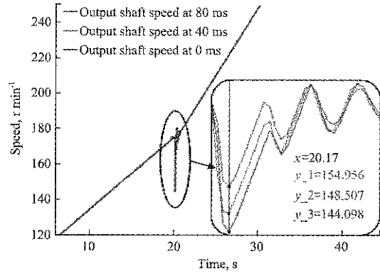
Figure 9 Different overlapping shift time in AMESim simulation model (Speed-Time)
