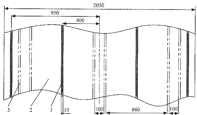
1. Reinforcement rib 2. Ordinary plastic film 3. Row spacing
