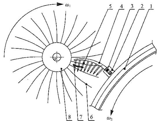
1. Nail tooth roller 2. Nail seat 3. Connecting piece 4. Main nail teeth 5. Small nail teeth 6. Brush 7. Plastic film 8. Brush roller
