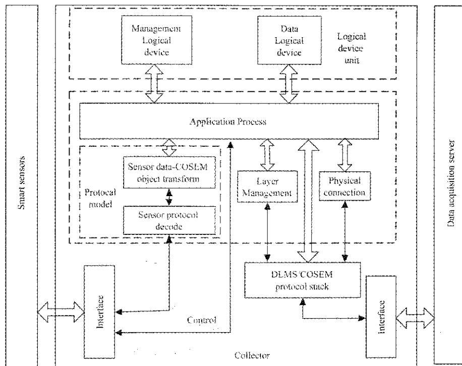
Figure 2 System architecture
