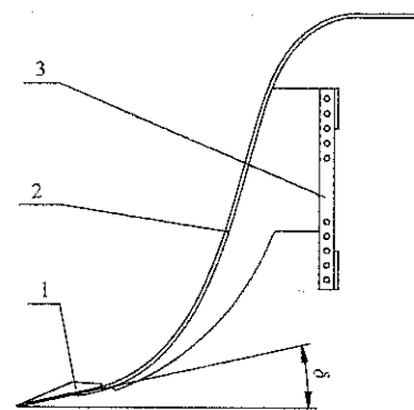
1. Loosening shovel 2. Handles 3. Depth adjustment plate 4. Rakeangle
