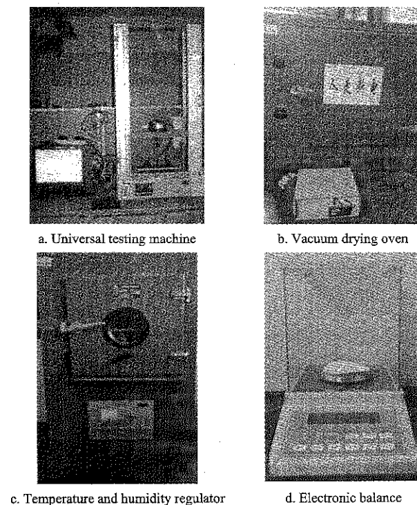
Figure 3 Test equipment
