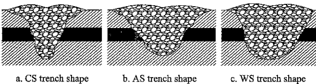
Figure 4 Subsoiling trench shape of different subsoiling tines
