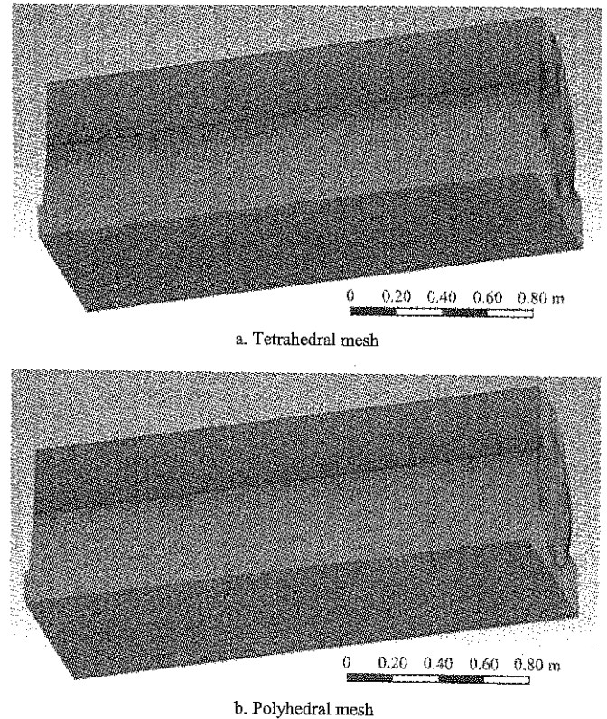
Figure 5 Grid generation for three-dimensional chopping chamber
