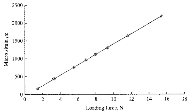
Figure 8 Calibration curve
