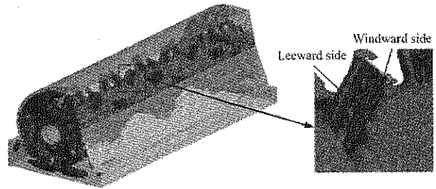
Figure 8 Core vortex regions in the chopping chamber
