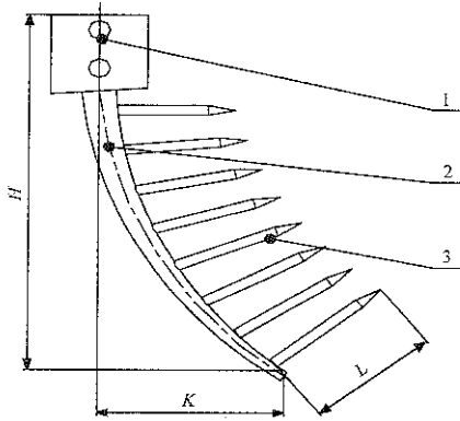
1. Mounting plate 2. Main nail teeth 3. Small nail teeth Figure 4 Sketch of nail teeth
