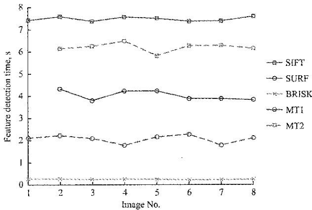
Figure 6 Different algorithm for feature detection, matching time
