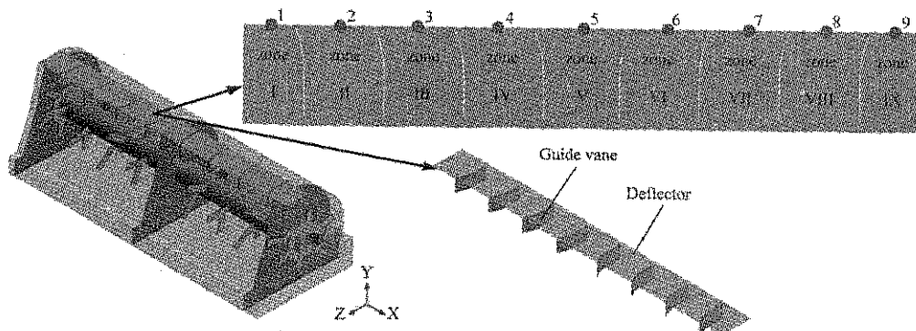
Figure 16 Computational domain of 9 zones (I-IX) and sampling points 1-9 of a chopping chamber fitted with guide vanes
