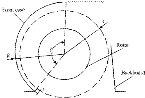
Figure 2 Structural parameters of the curved front case
