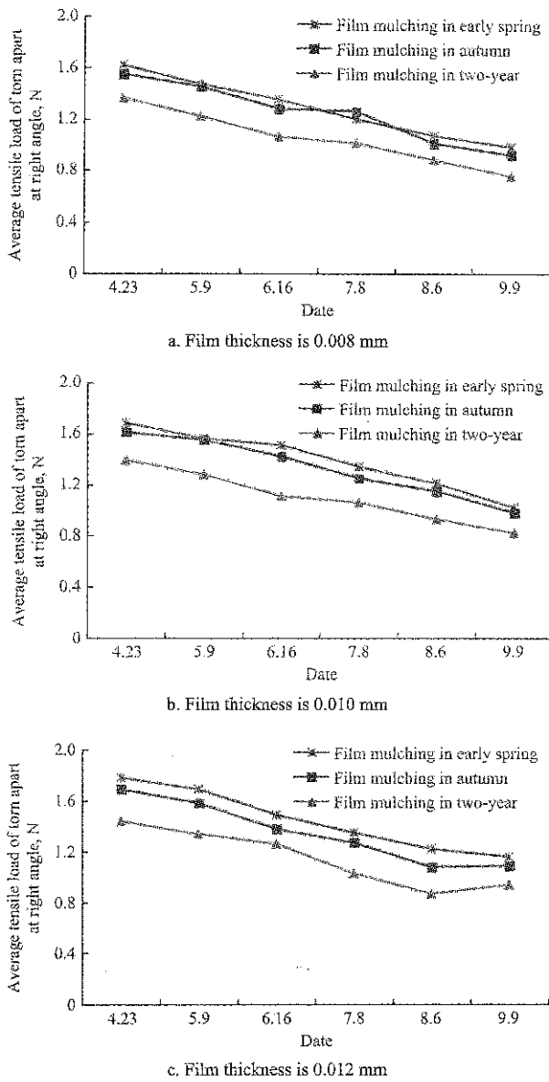
Figure 8 Average tensile load of torn apart at right angles in corn growth stage
