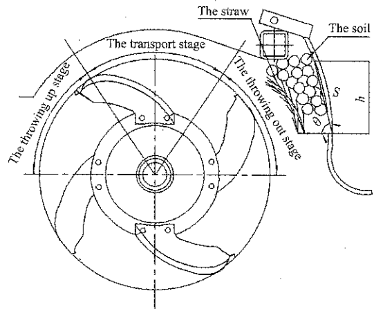
Figure 7 Process of soil covers rice whole straw
