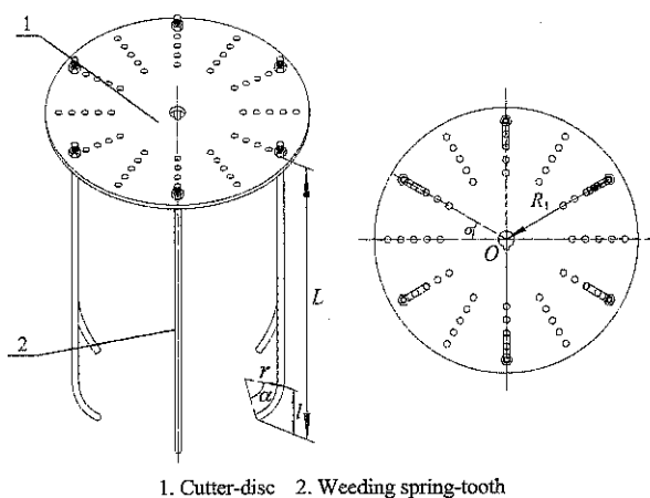
Figure 2 Rotating and burying weeding device for paddy field
