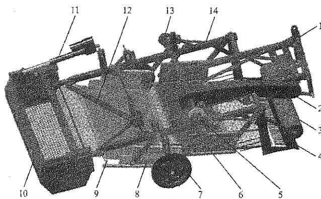
1. Hitch frame 2. Transmission device 3. Soil-breaking roller 4. Digging shovel 5. Vibration driving device 6. Fore-screen 7. Depth stop 8. Back-screen 9. Ball stud 10. Film-collecting basket 11. Unloading device 12. Soil-guiding device
