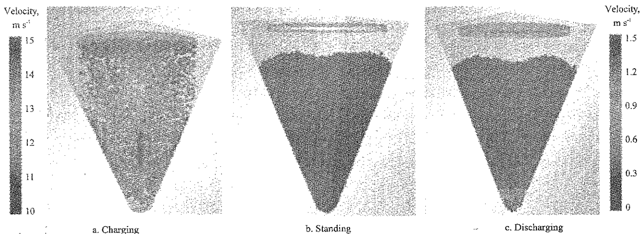
Figure 4 Charging and discharging processes of the pyramidal funnel
