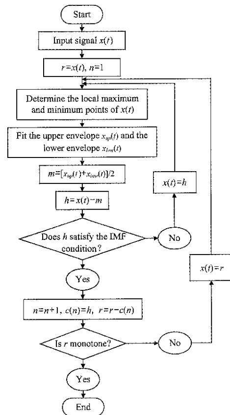
Figure 1 Decomposition flow chart of EMD
