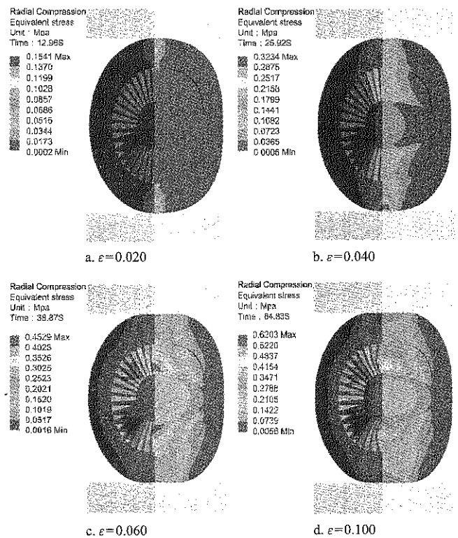
Figure 9 Stress nephogram of radial compression
