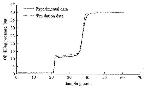
Figure 7 Comparison of experimental and simulated results of clutch in AMESim
