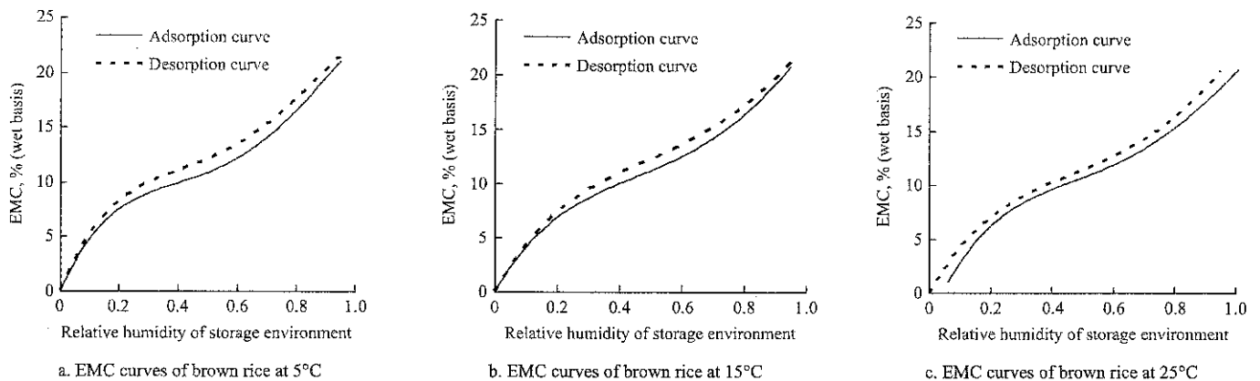
Figure 1 EMC curves of brown rice at three different temperatures
