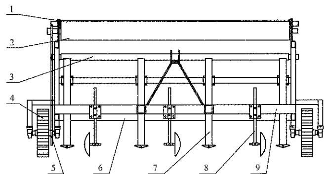
1. Film rolling unit and a film unloading unit 2. Supporting unit 3. Film unfolding unit 4. Ground wheels 5. Frame 6. Power transmission system 7. Loosening shovel unit 8. Film slitting unit 9. Suspension unit
